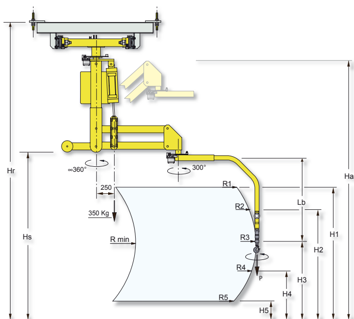
PARTNER PM overhead trolley mounted "PMS"
