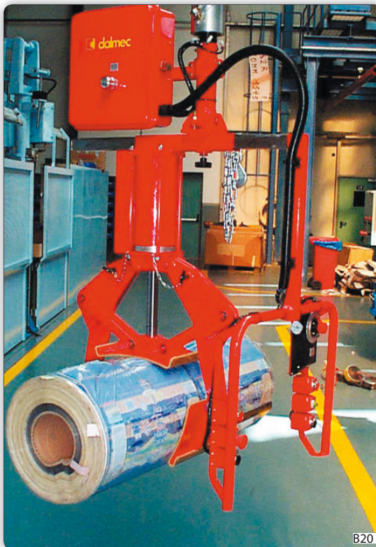
Manipulator fitted with pneumatic grippers for handling reels about their outside diameter.
