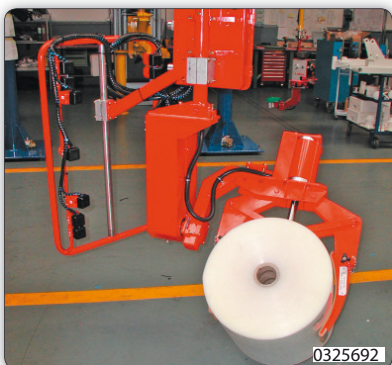
Gripper tooling with pneumatic rotation.
