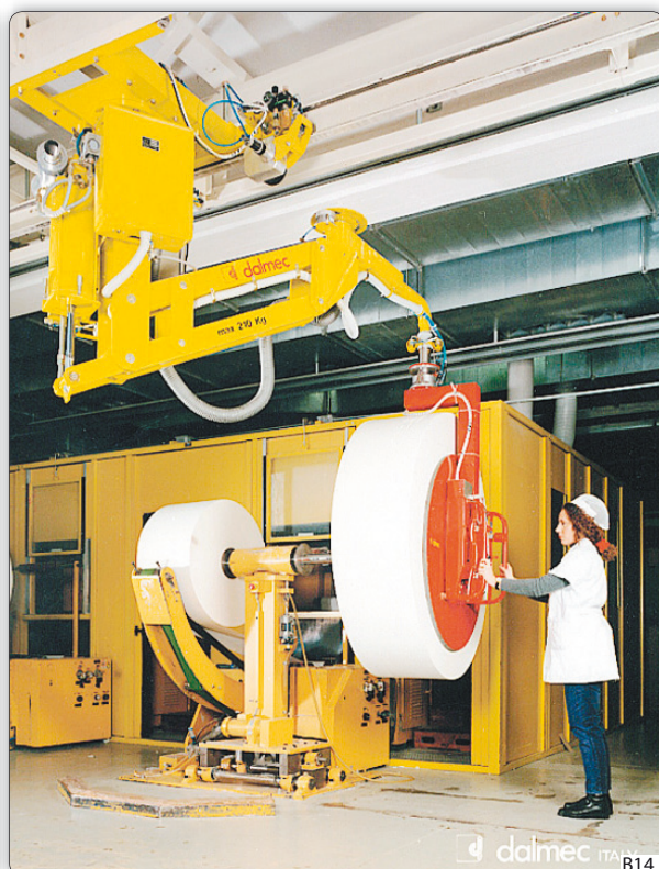
PMS type Partner manipulator, overhead trolley mounted, with pneumatic trolley drive, designed for the handling of reels of cardboard. The tooling comprises a suction head designed to pick reels from the floor and place them to the shaft of an unwinding machine. The vacuum is generated by a vacuum pump.
