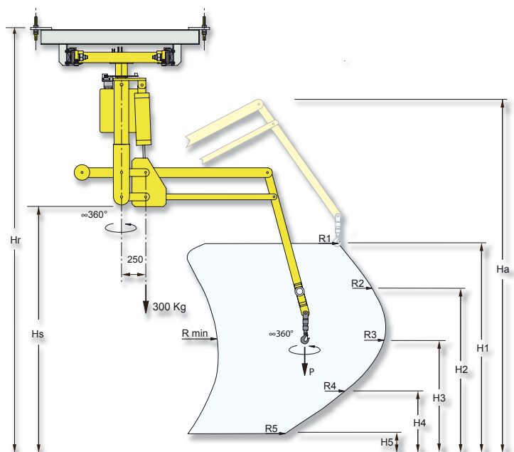
PARTNER PS overhead trolley mounted "PSS"
