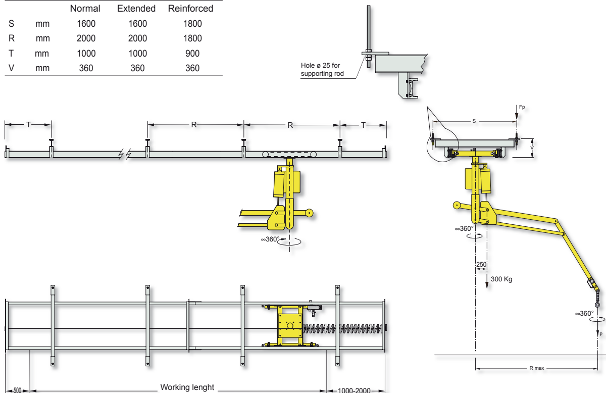
Tracks dimensions
